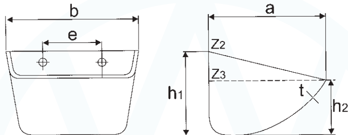
BE type plastic elevator buckets (parameters in mm)
