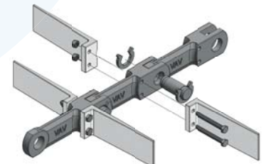
Easy to attache/detache plastic scrapers
